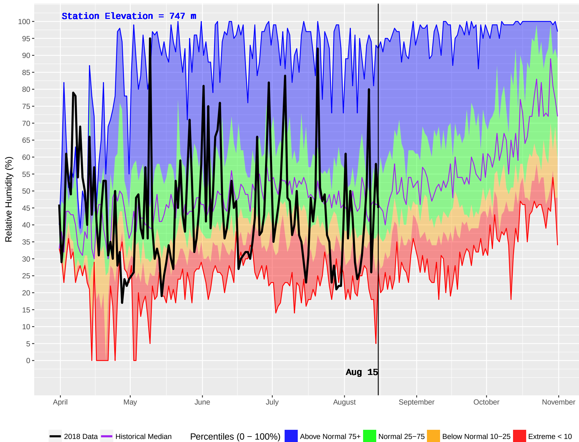
PEDEN (178) : Historical (1984–2016) and Current (2018) Daily Relative Humidity
