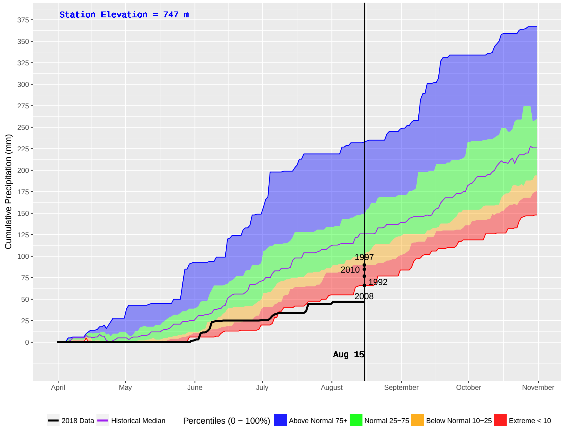
PEDEN (178) : Historical (1984–2016) and Current (2018) Daily Cumulative Precipitation
