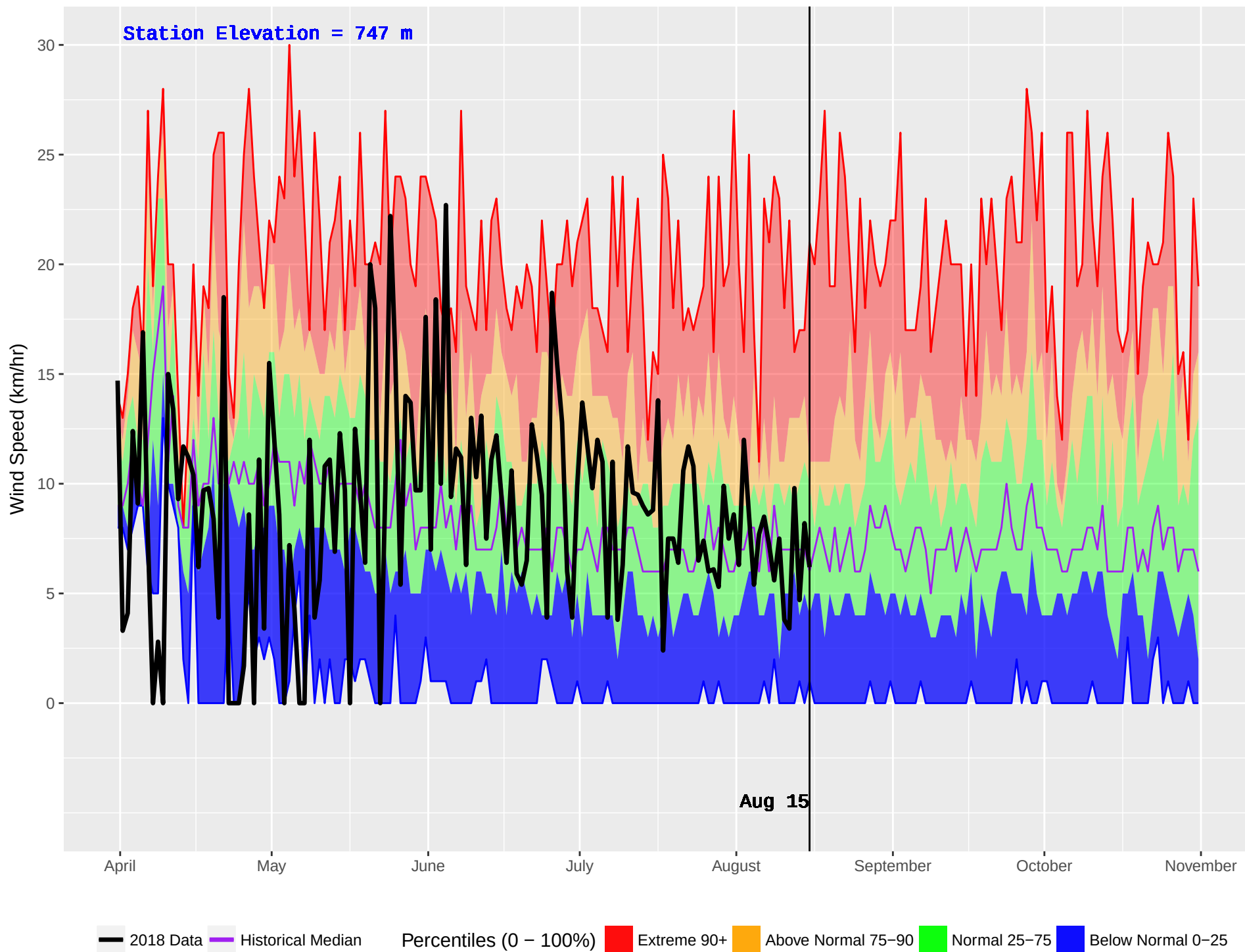
PEDEN (178) : Historical (1984–2016) and Current (2018) Daily Wind Speed
