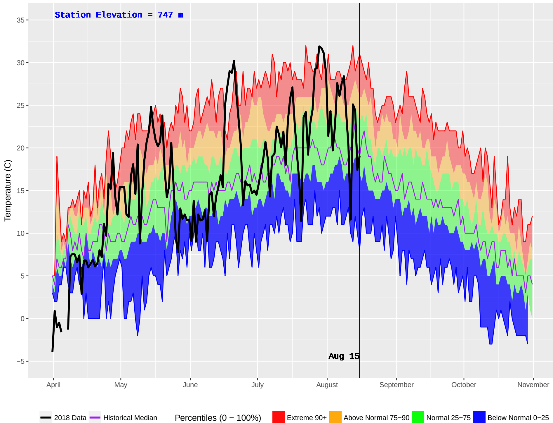
PEDEN (178) : Historical (1984–2016) and Current (2018) Daily Temperature
