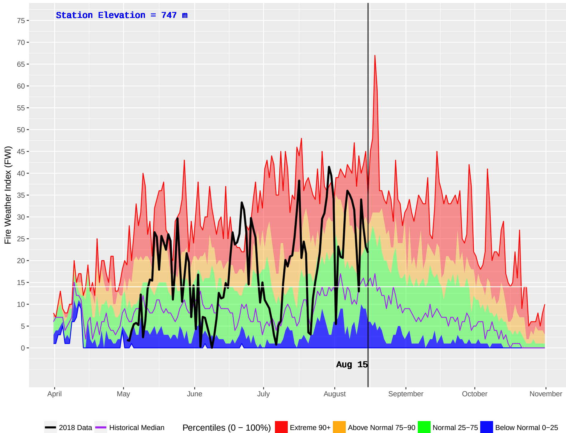
PEDEN (178) : Historical (1984–2016) and Current (2018) Daily Fire Weather Index (FWI)
