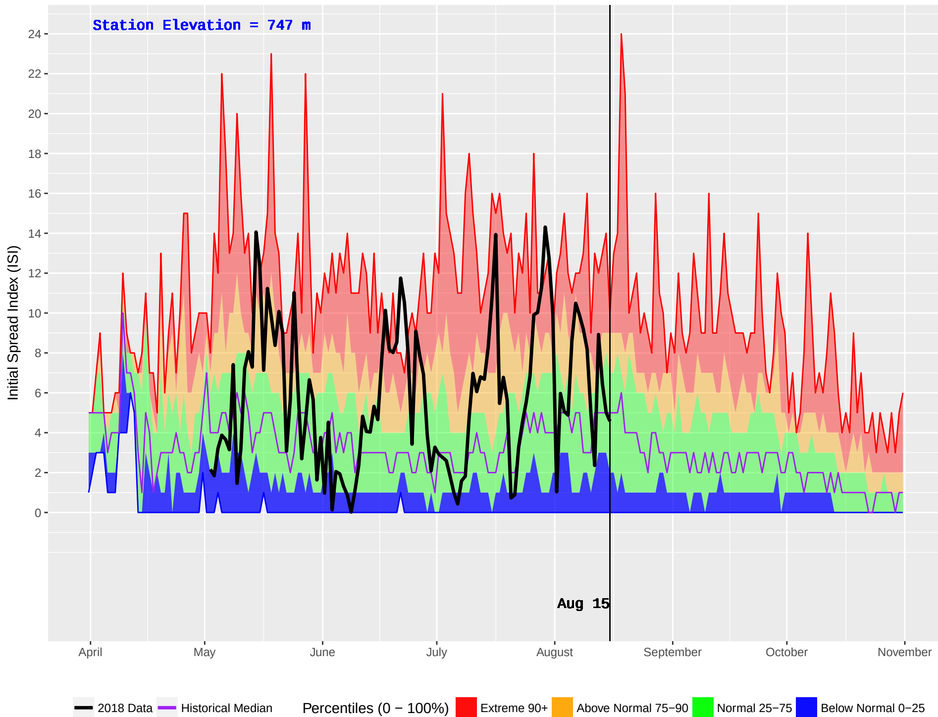
PEDEN (178) : Historical (1984–2016) and Current (2018) Daily Initial Spread Index (ISI)
