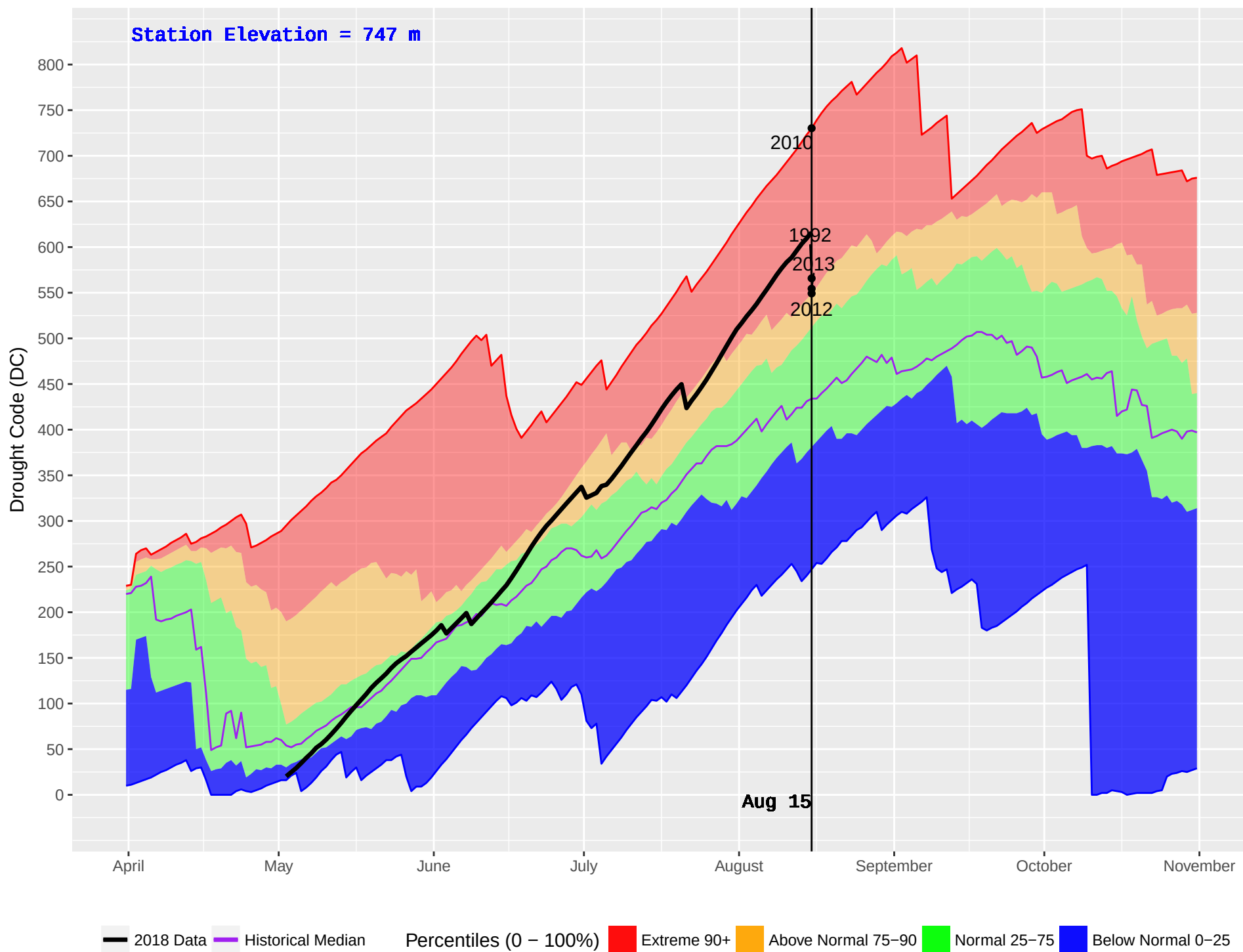
PEDEN (178) : Historical (1984–2016) and Current (2018) Daily Drought Code (DC)
